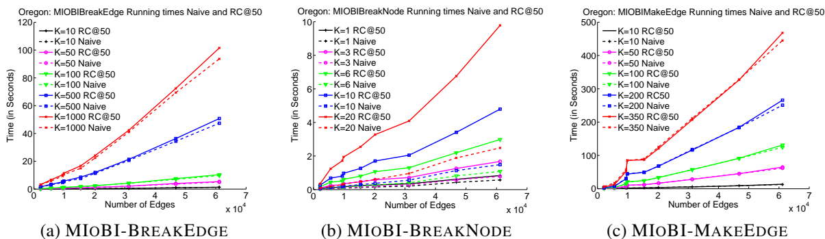
Figure 2: Scalability of proposed methods: all three algorithms scale near-linearly wrt graph size. (figures best in color)
