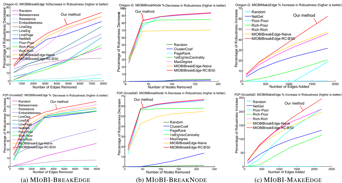
Figure 1: % robustness change (higher is better) vs. budget k for proposed MIOBI and various competing heuristics on two datasets, (top) Oregon-G and (bottom) P2P-GnutellaD , for (a) edge deletions, (b) node deletions, and (c) edge additions. Notice that our methods outperform all the heuristics at all ranges of k . (figures best viewed in color)
